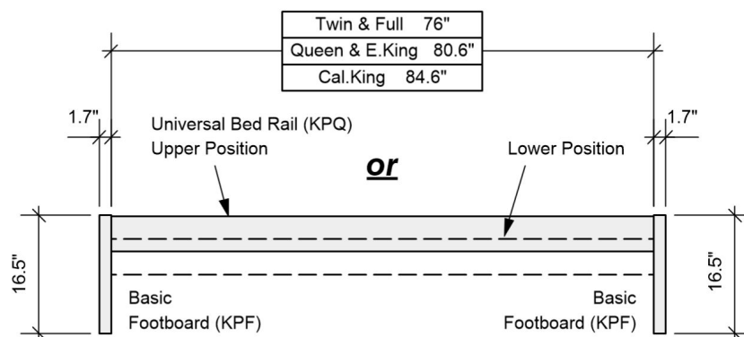
Rails Side View
